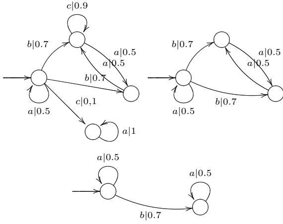
Fig. 2: Processes P , P|_\sigma and Q .
