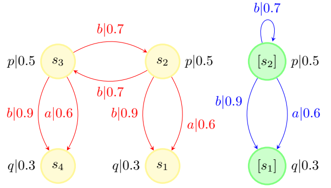
Fig. 1: Construction of a quotient model.
